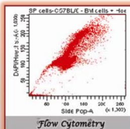
Flow Cytometry
