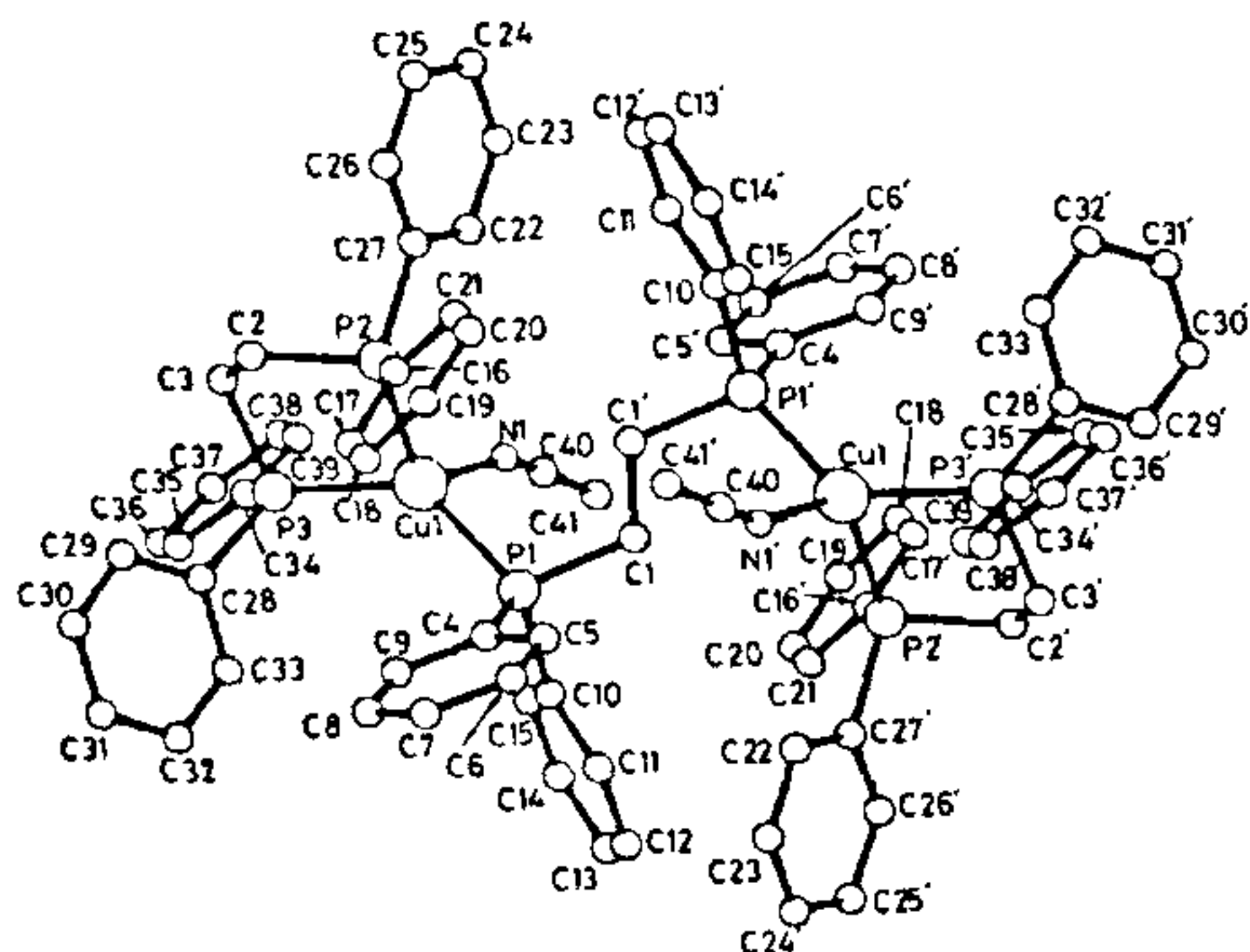
Figure 2. PLUTO diagram of the complex 3.
