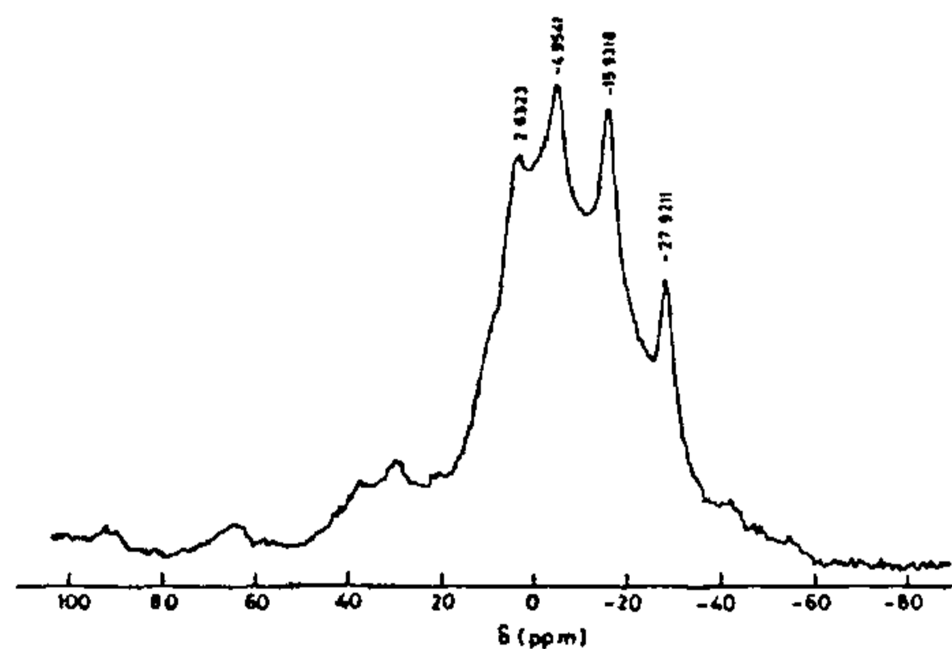
Figure 3. Solid state CP/MAS ^{31}\text{P} NMR spectrum of complex 1.
