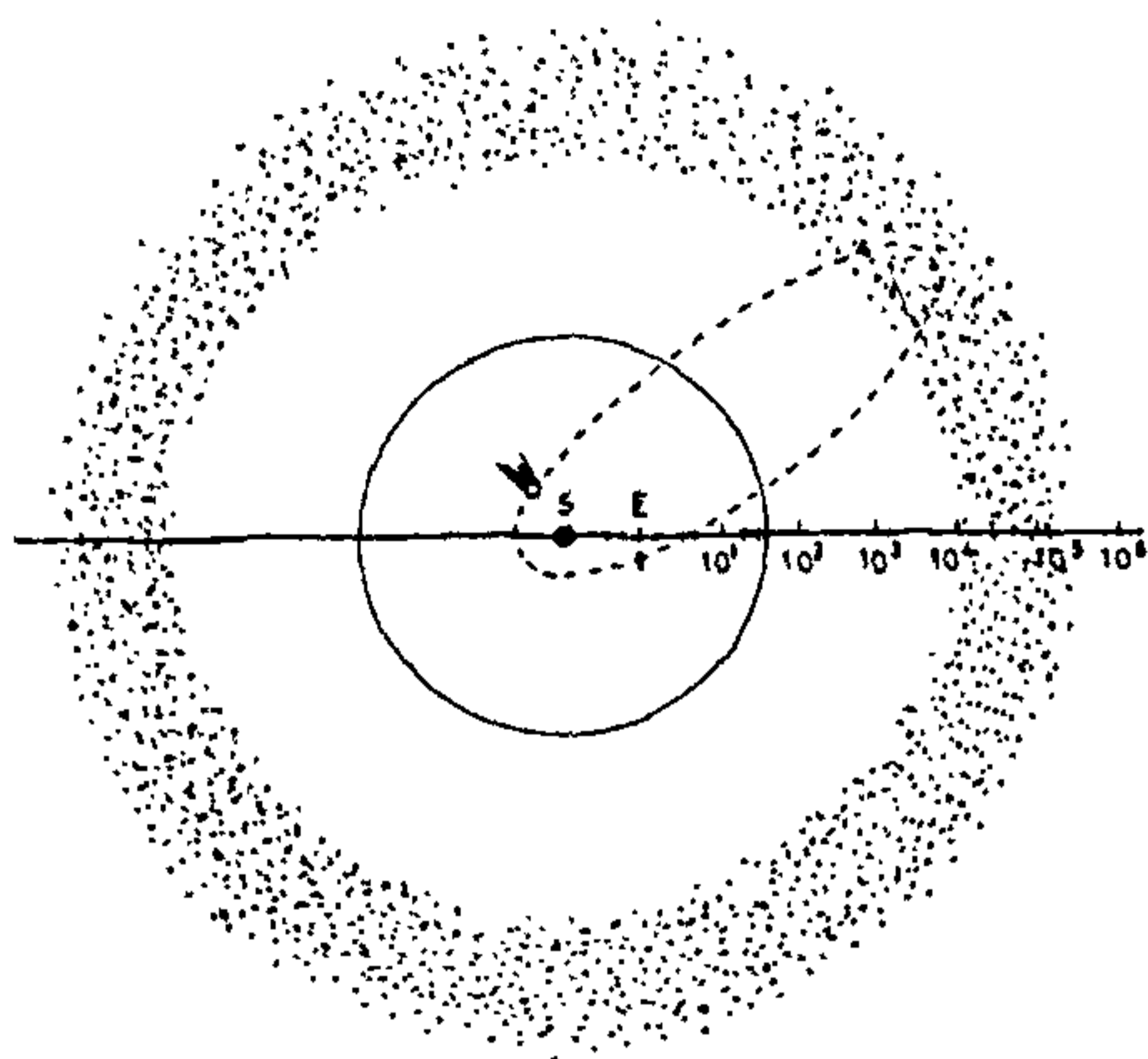
Figure 1. The Oort comet cloud is shown schematically. The radial dimensions are logarithmic in astronomical units. The planetary system is encircled and the relative positions of the Sun (S), Earth (E) and other planets are marked. A long-period comet on an elliptic orbit is also shown.
