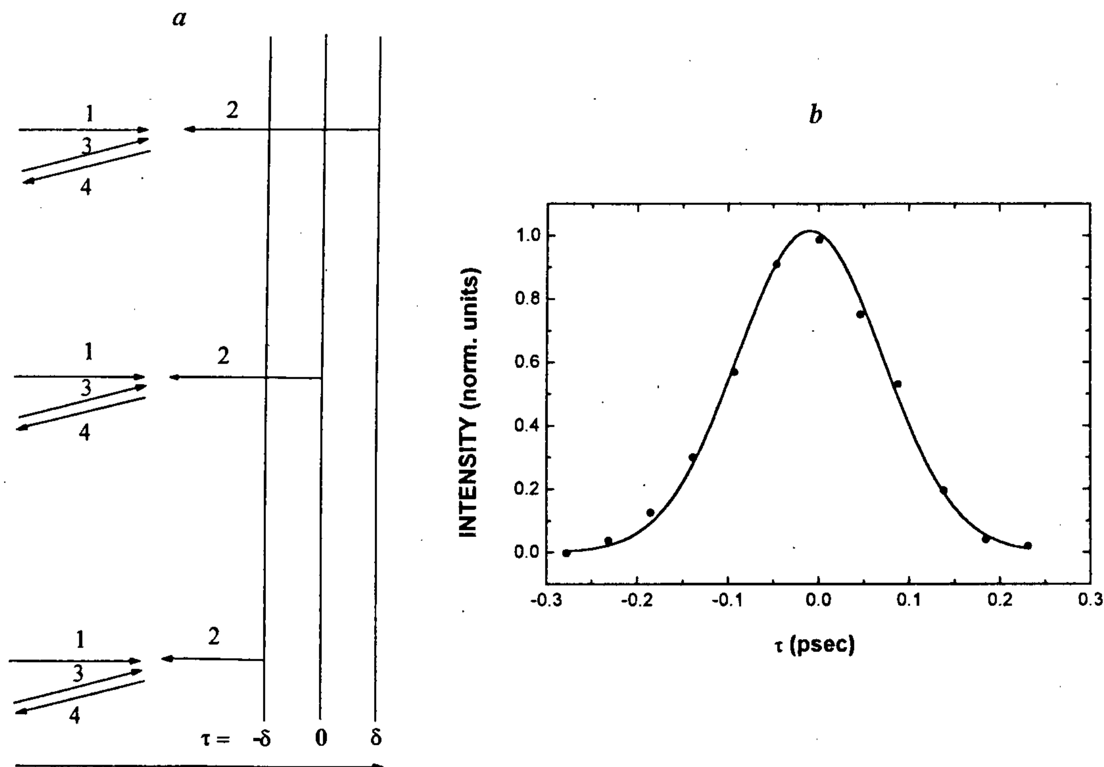
Figure 3. a , Pictorial representation of various delays. b , Autocorrelation function (RhB in methanol).
