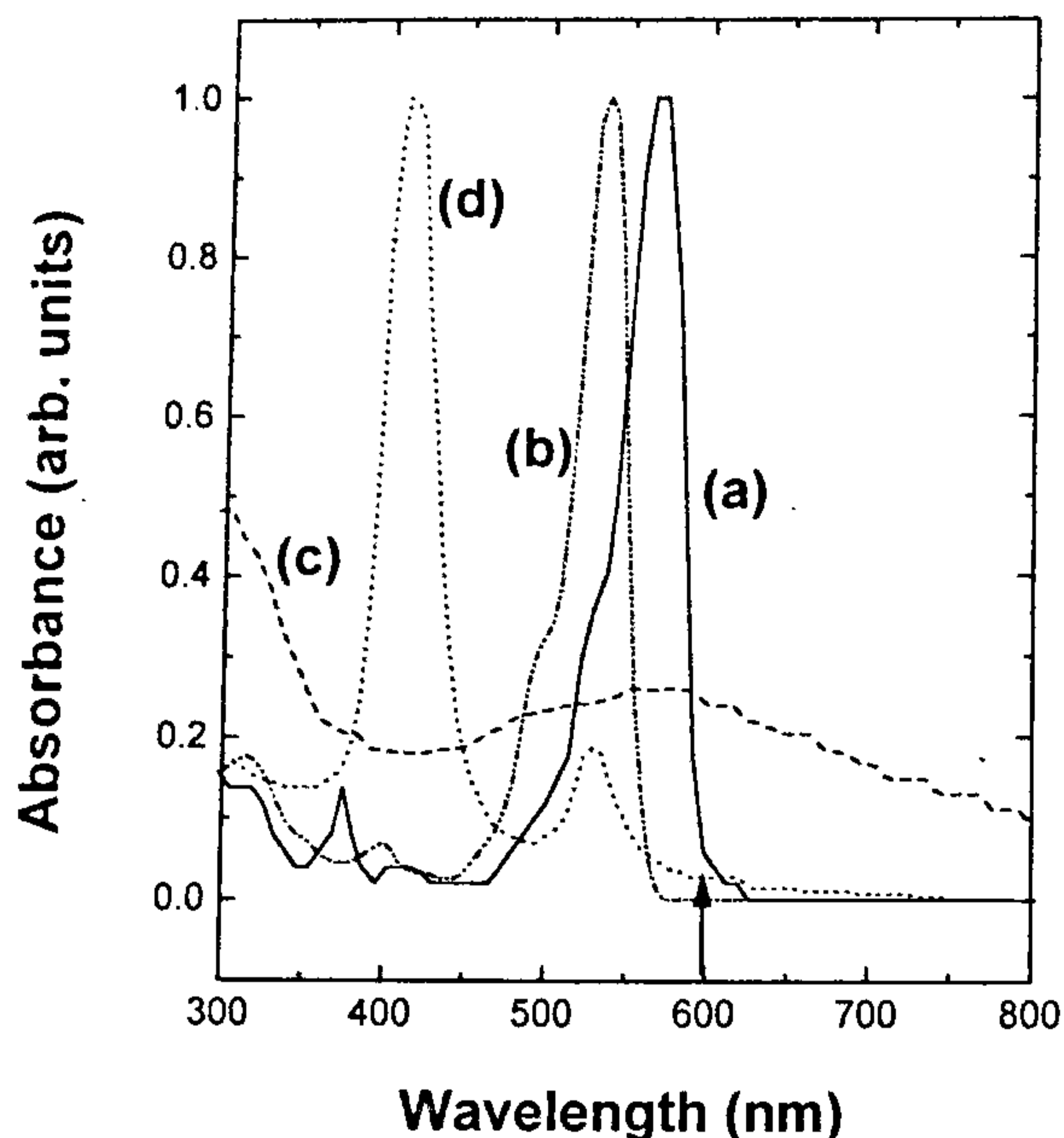
Figure 2. Absorption spectrum of the samples. a , RhB; b , erythrosinB; c , black ink; d , CoTTP.
