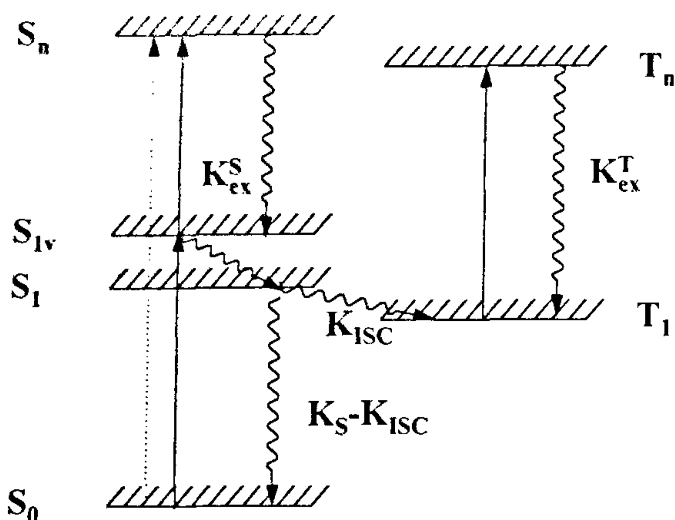
Figure 5. Energy level structure in organic molecules indicating different transitions.
