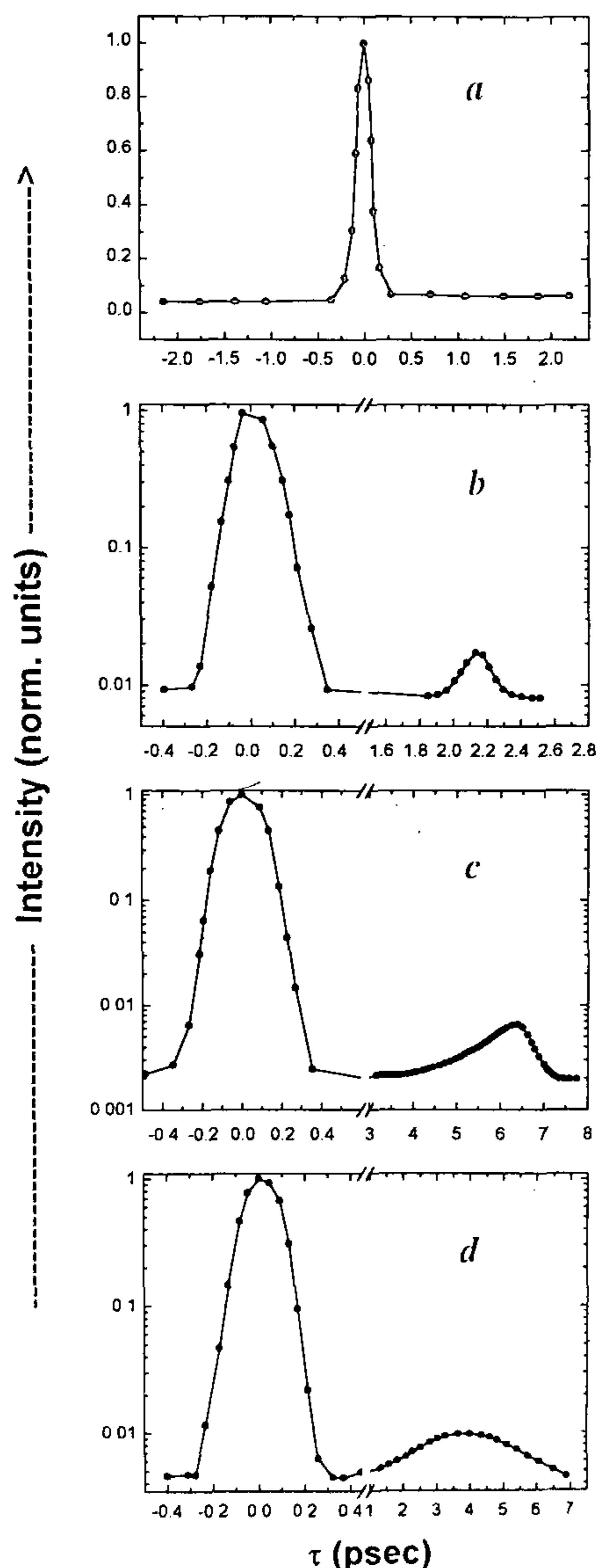
Figure 4. a, Signal profile for \delta = 1 ps in sample RhB in methanol; b, signal profile for \delta = 2.1 ps in sample erythrosinB in methanol; c, signal profile for \delta = 6.4 ps in sample black ink in distilled water; d, signal profile for \delta = 4 ps in sample CoTTP.
