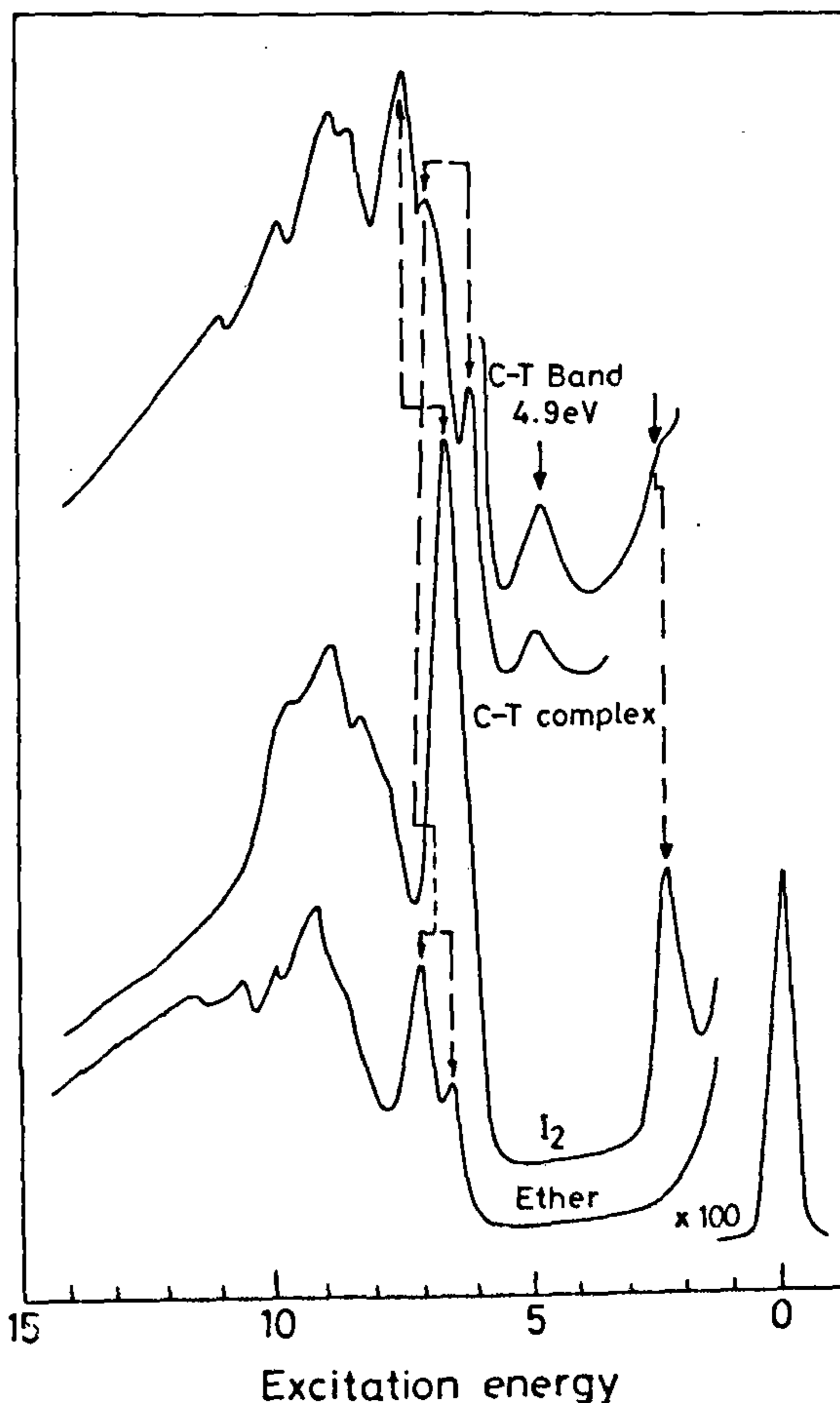
Figure 9. Electron energy loss spectra of ether, I_2 and their complex.
