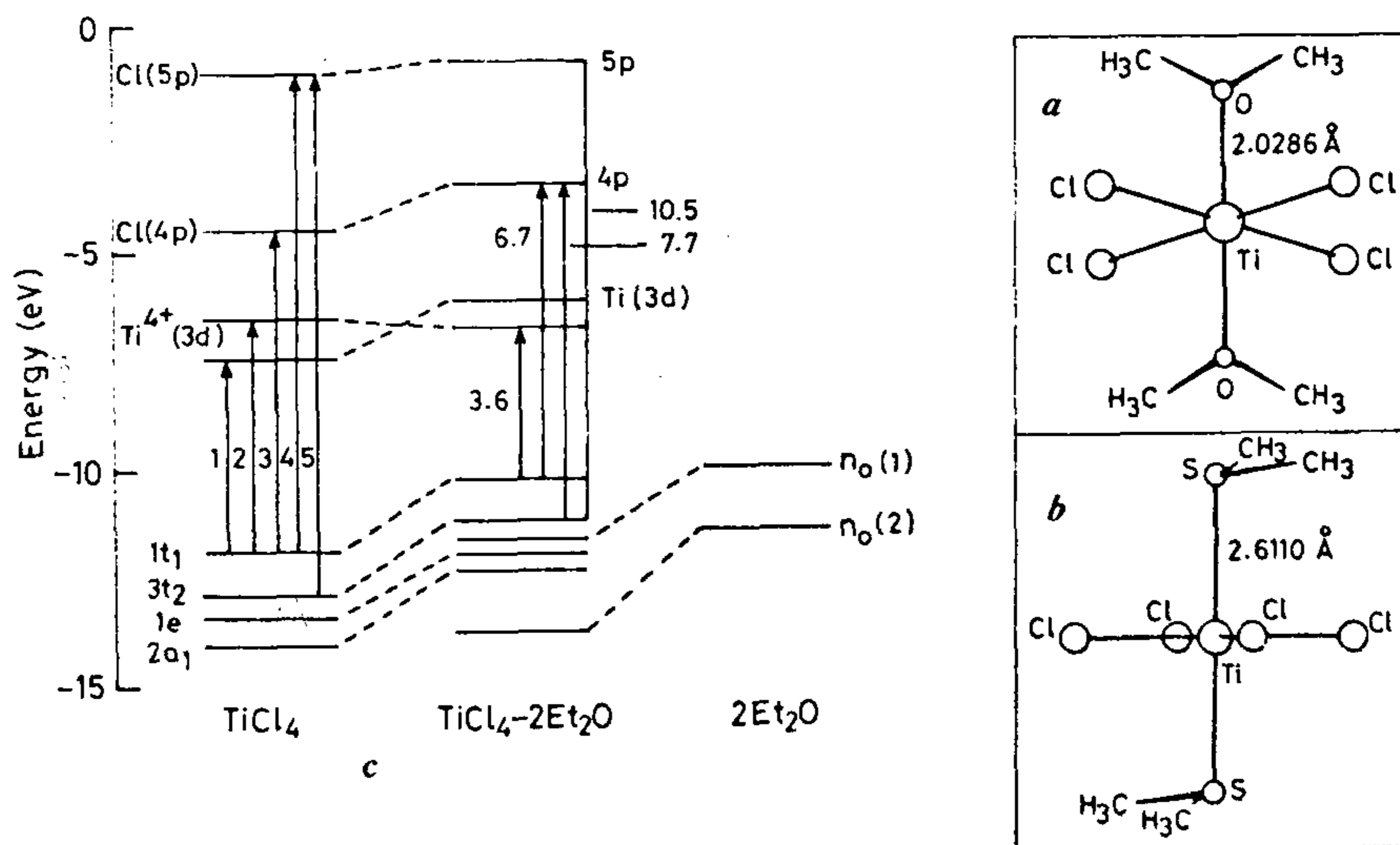
Figure 14. (a) and (b) optimized geometry of \text{TiCl}_4 complexes. (c) Electron states of \text{TiCl}_4-2(\text{C}_2\text{H}_5)_2\text{O} complex.
