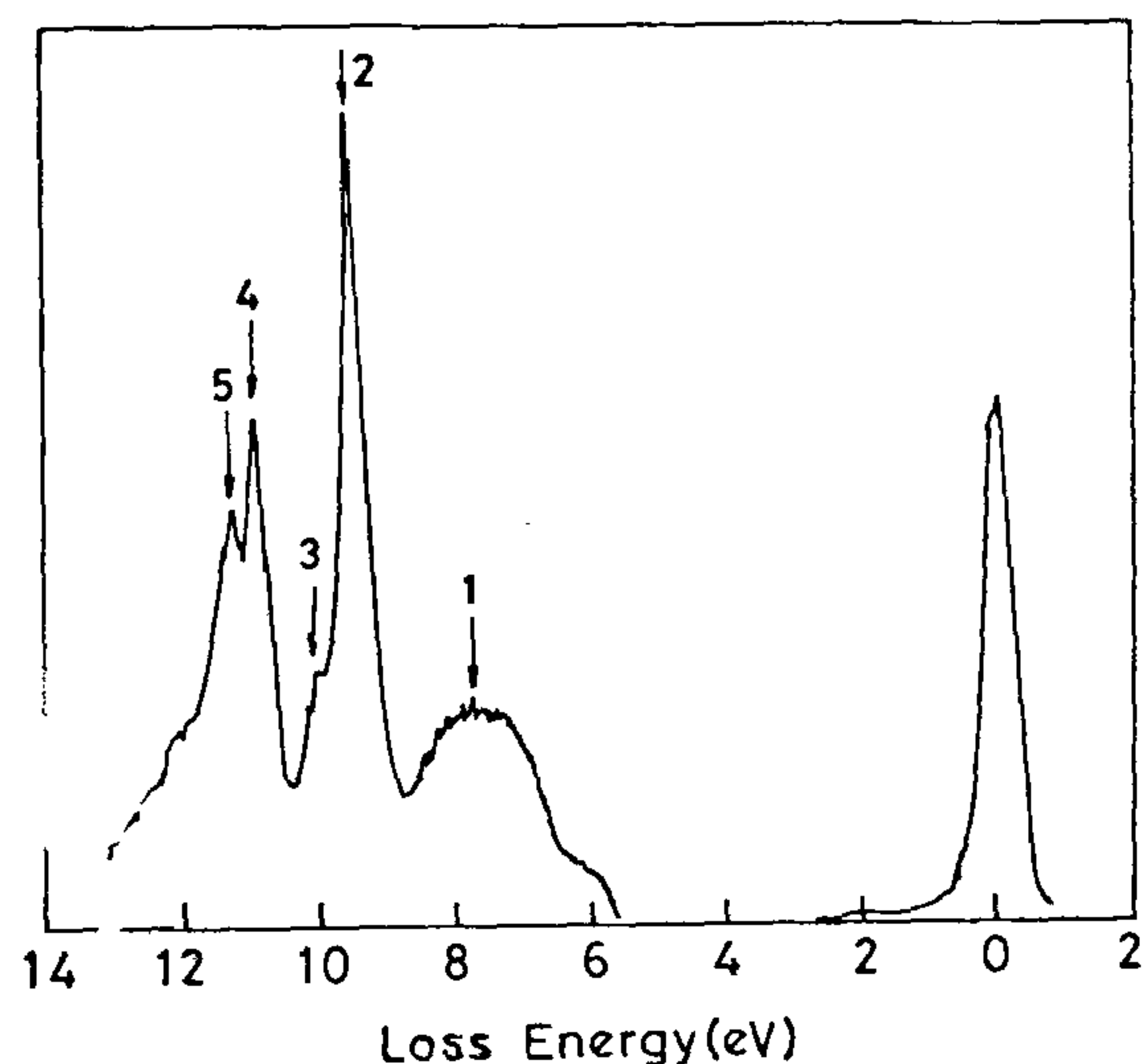
Figure 2. Electron energy loss spectrum of HCl.
