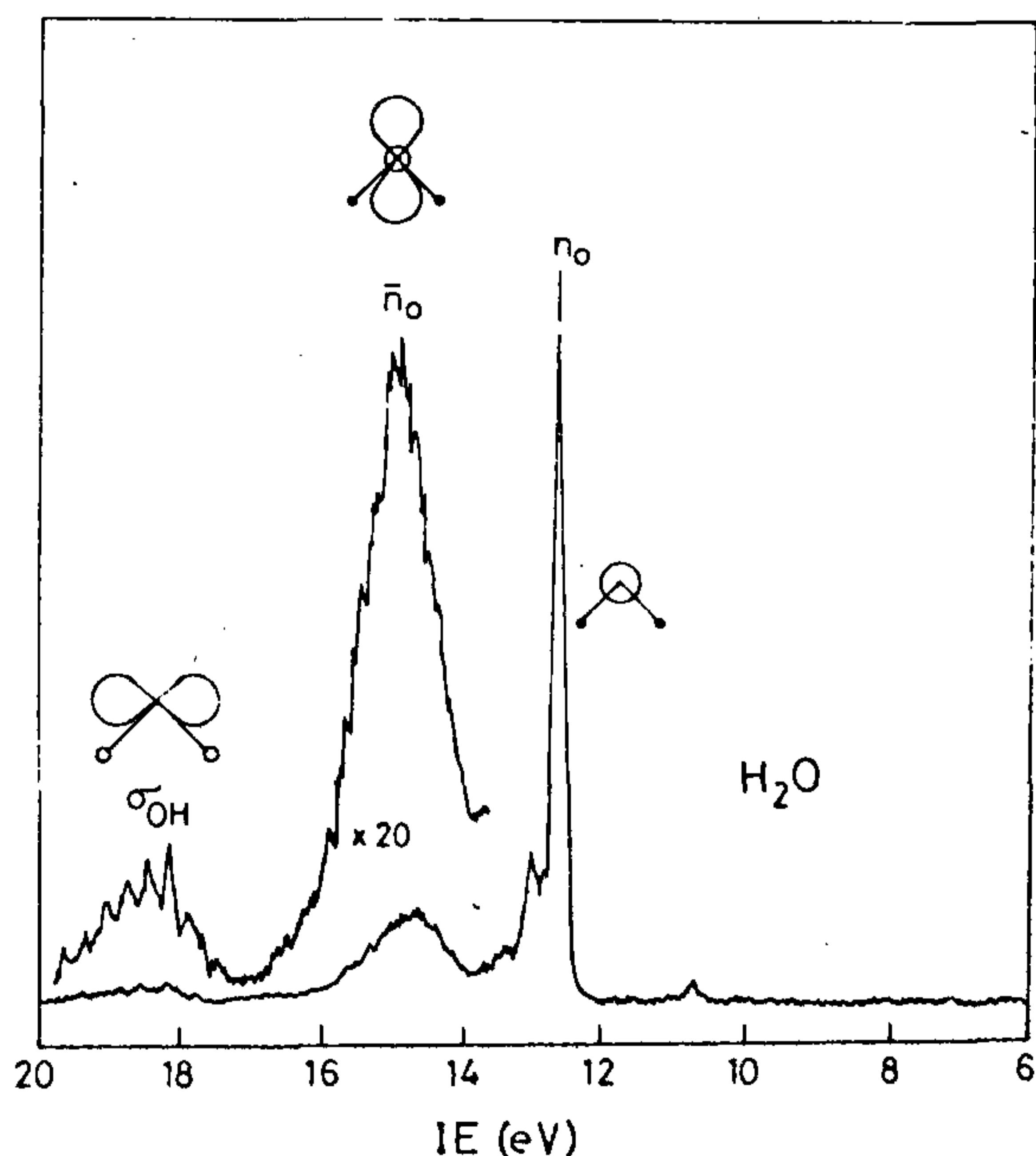
Figure 4. HeI photoelectron spectrum of H 2 O molecule.
