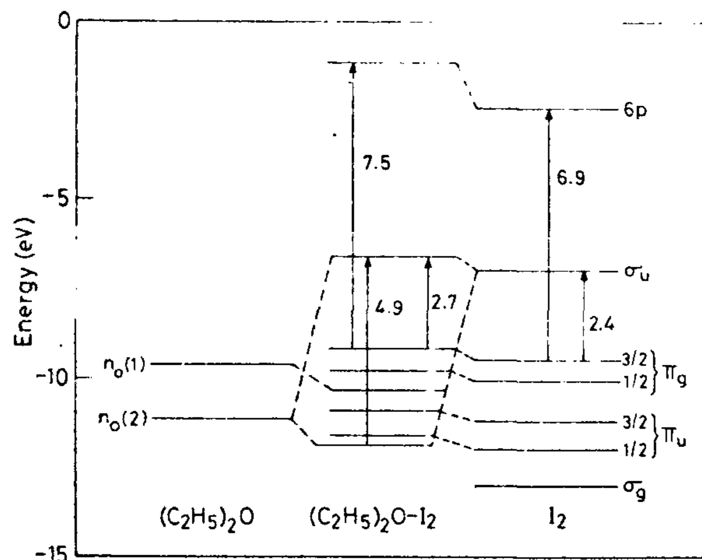
Figure 10. Electron states of ether, I_2 and their C-T complex.
