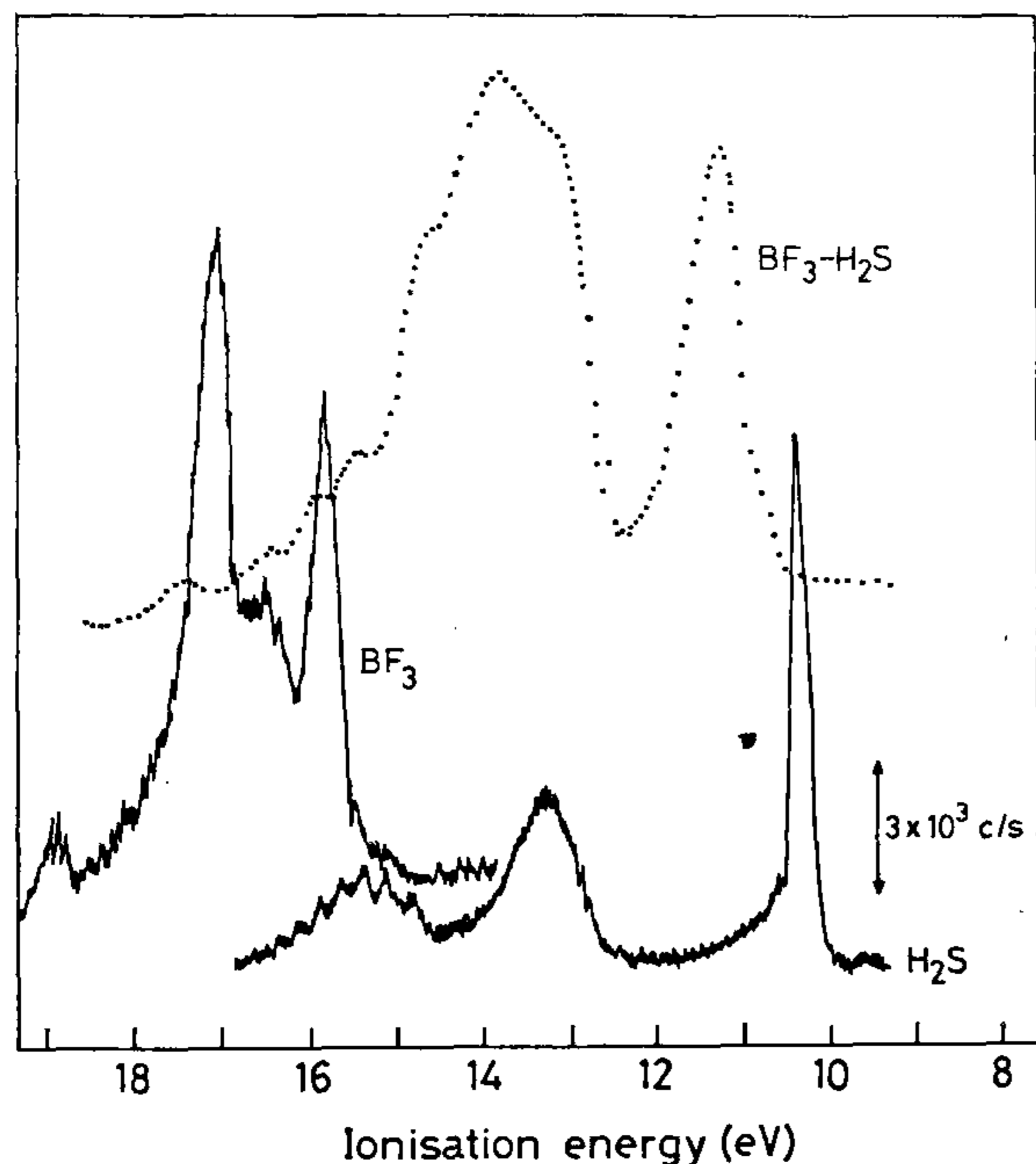
Figure 13. Hel UVPES of \text{BF}_3 , \text{H}_2\text{S} and their complex.
