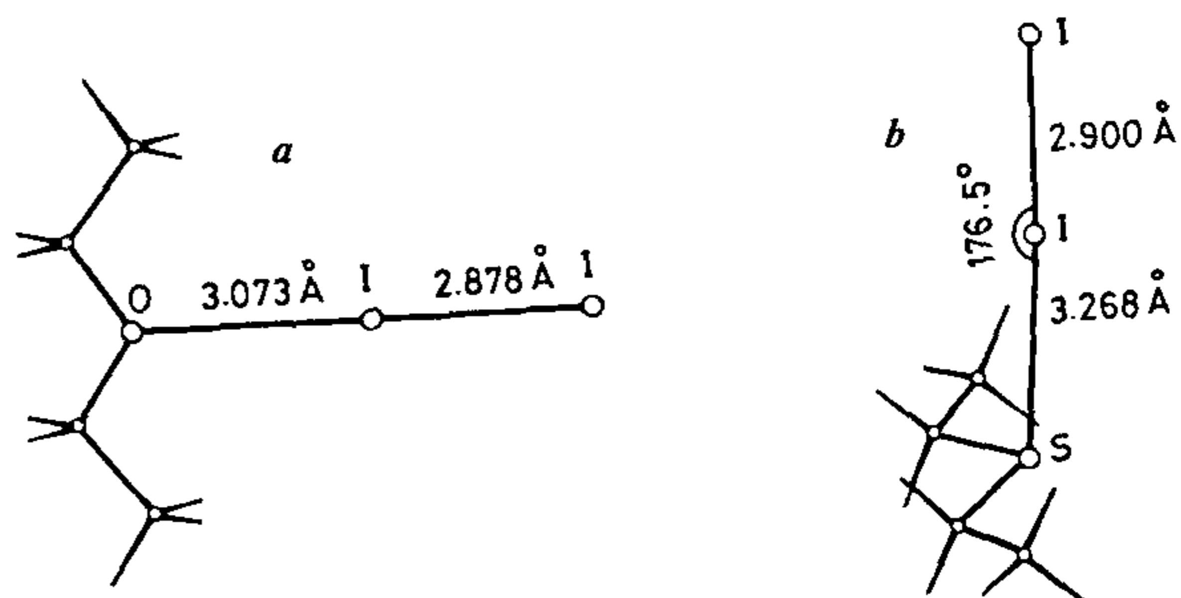
Figure 8. Optimized molecular geometry of (C_2H_5)_2O-I and (C_2H_5)_2S-I_2 .
