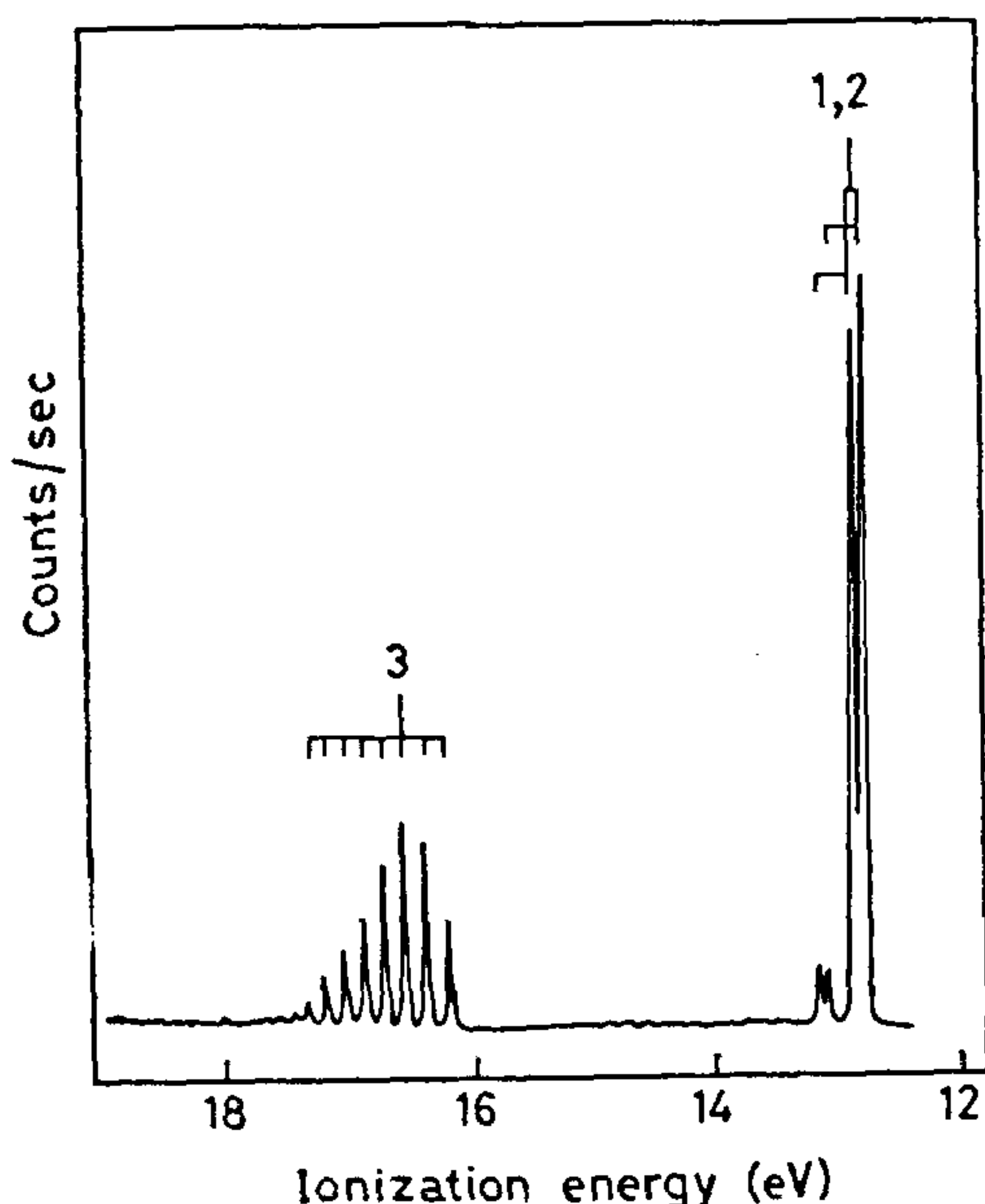
Figure 1. HeI photoelectron spectrum of HCl.
