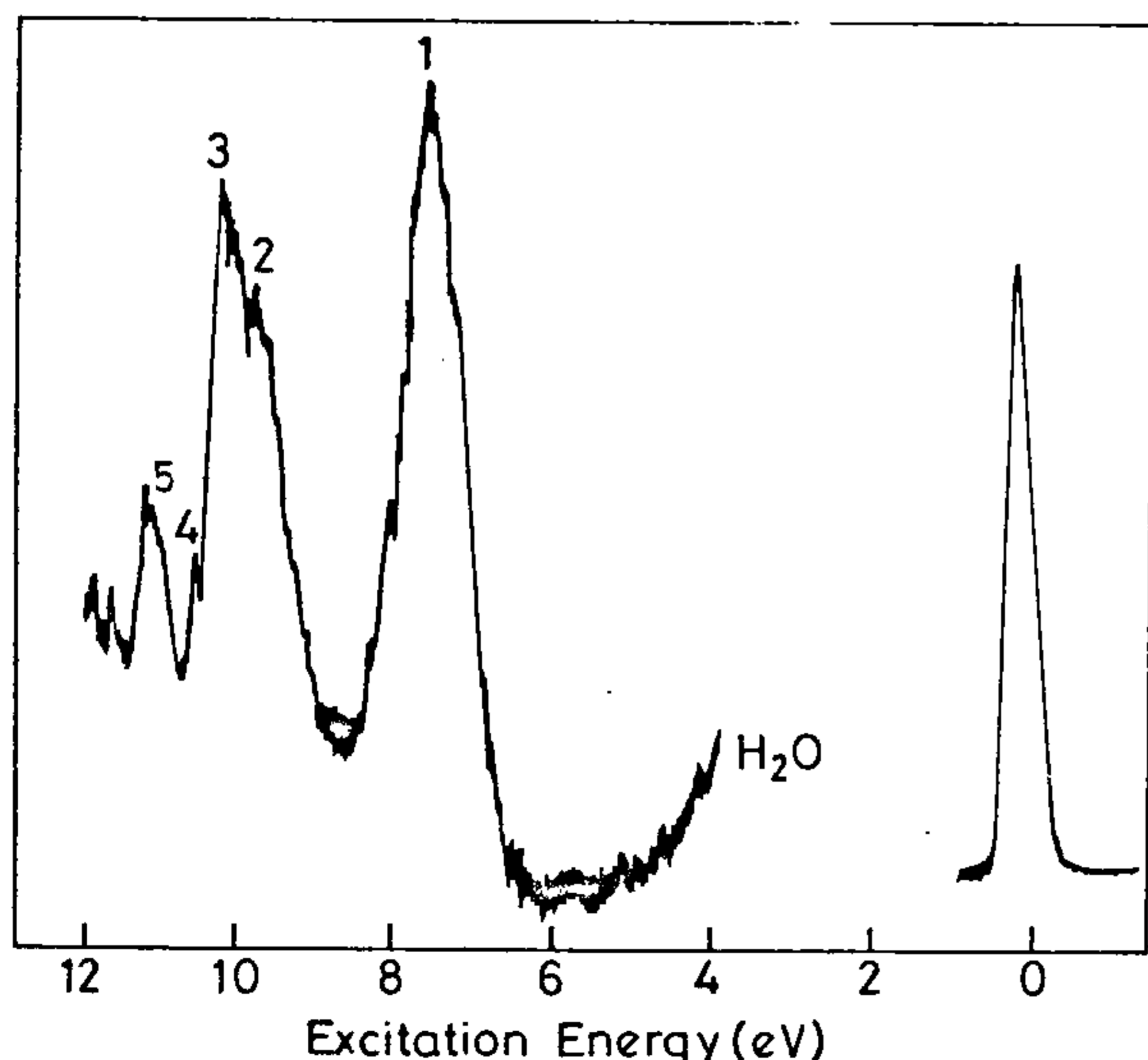
Figure 5. Electron energy loss spectrum of H 2 O.
