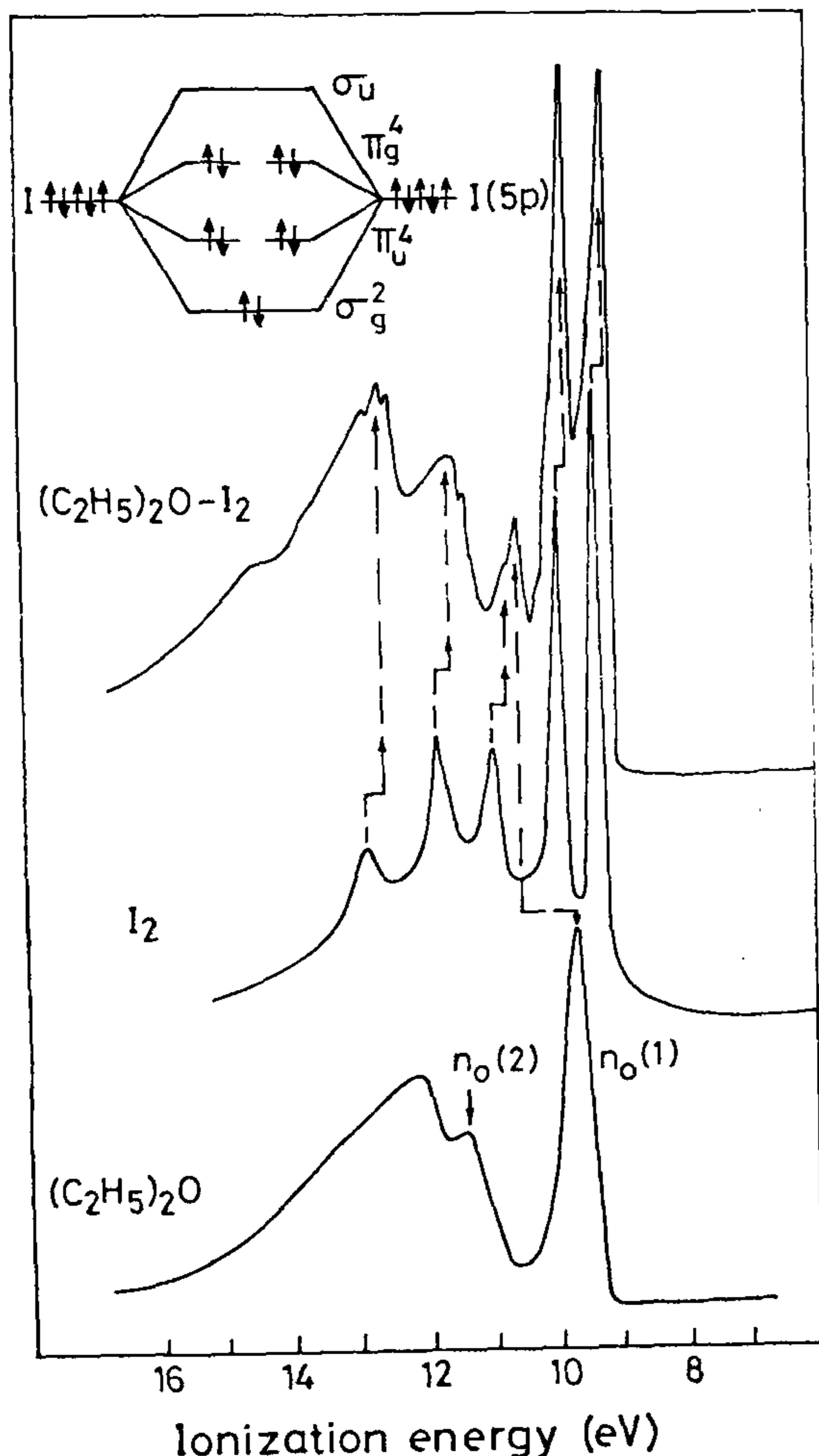
Figure 7. Hel UV photoelectron spectra of diethyl ether, iodine and their C-T complex.
