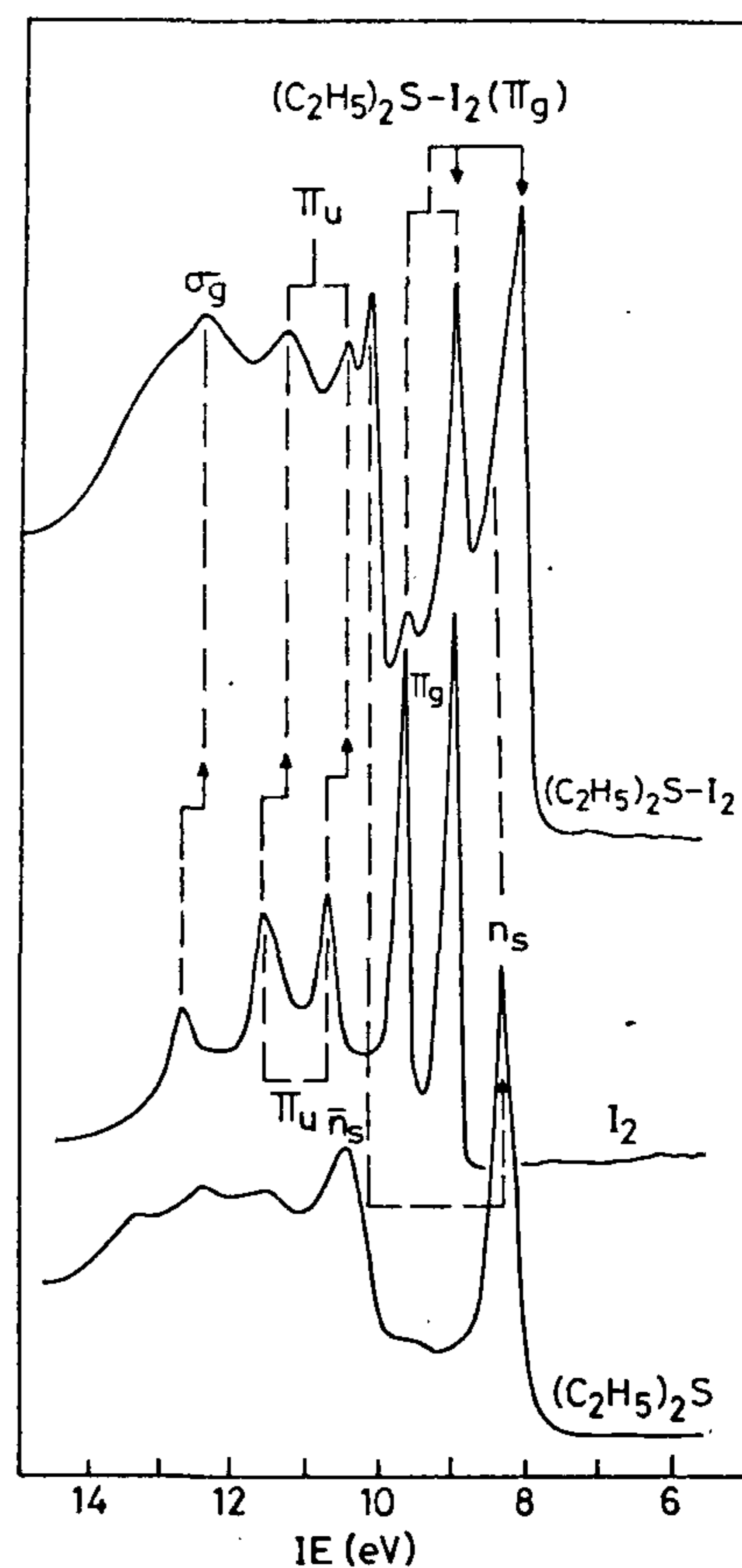
Figure 11. UVPES of diethyl sulphide, I_2 and their C-T complex.
