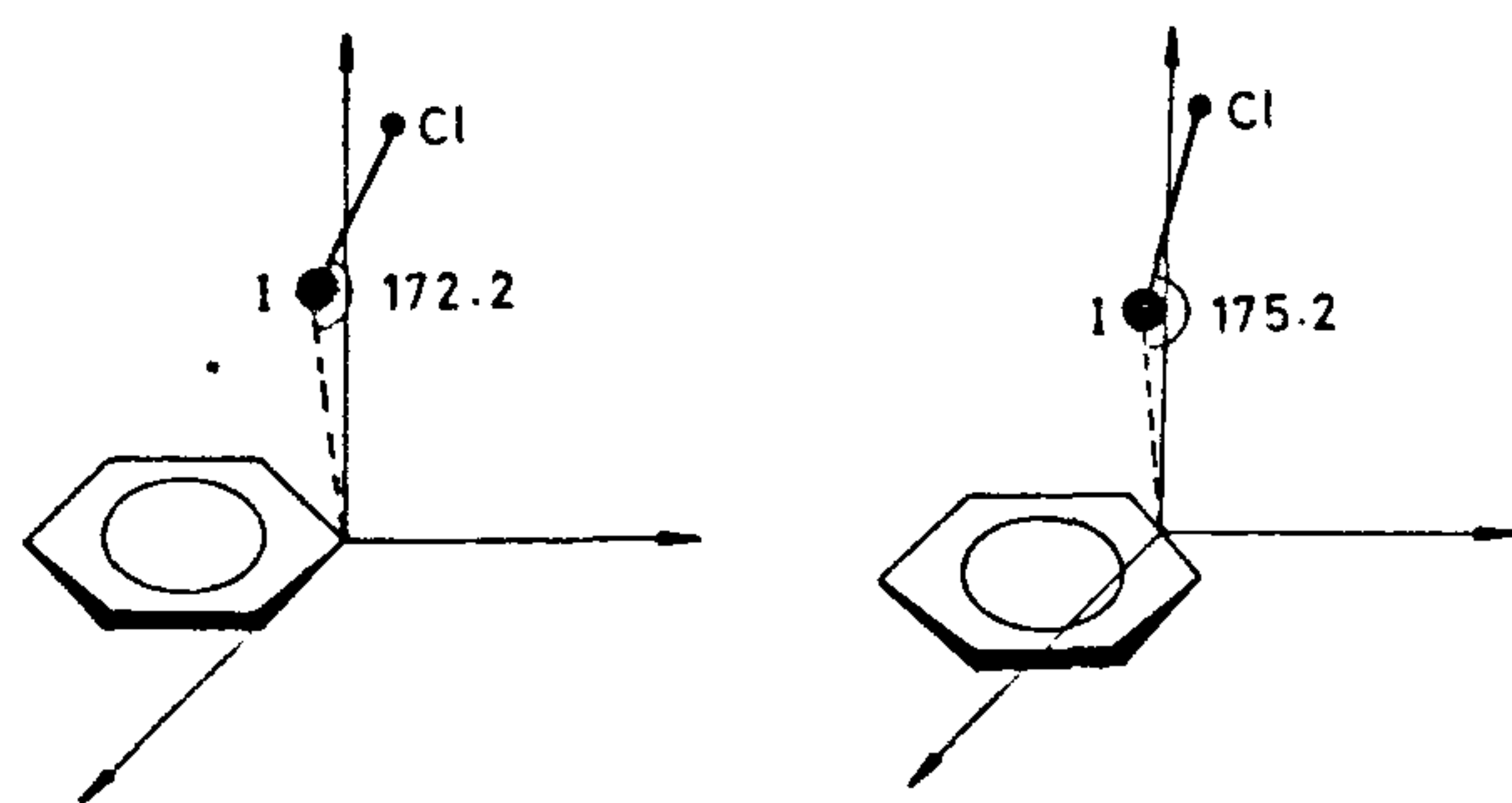
Figure 15. Optimized geometry of C_6H_6-ICl complex.
