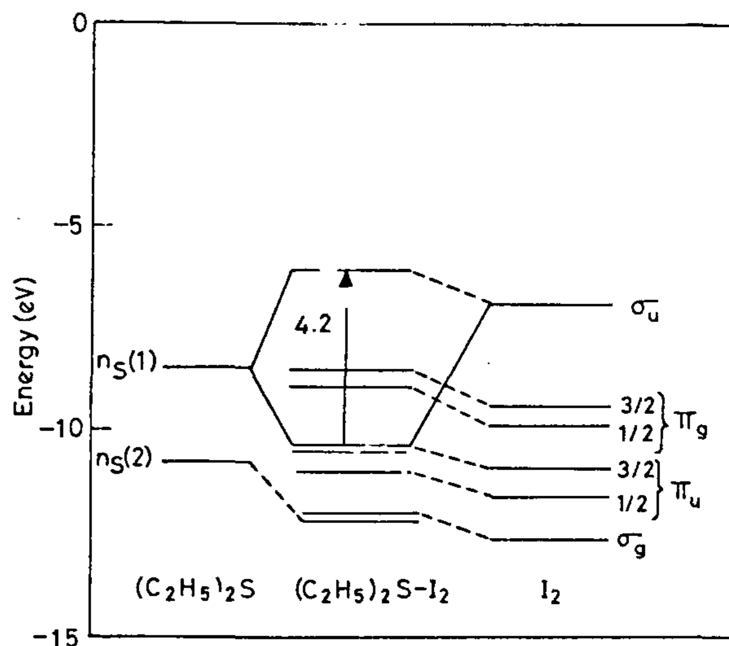
Figure 12. Electron states of diethyl sulphide- I_2 complex.
