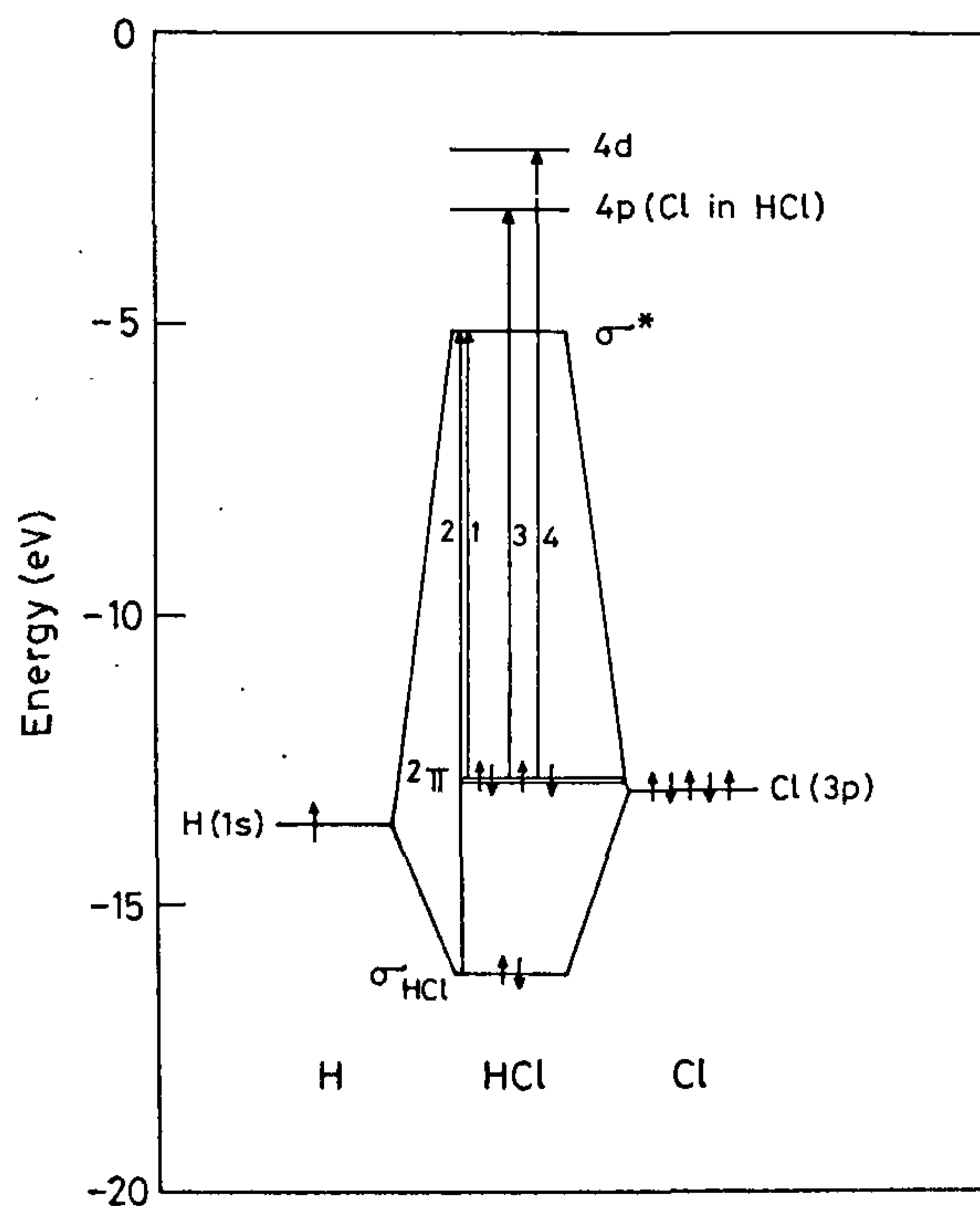
Figure 3. Energy level diagram of HCl molecule.
