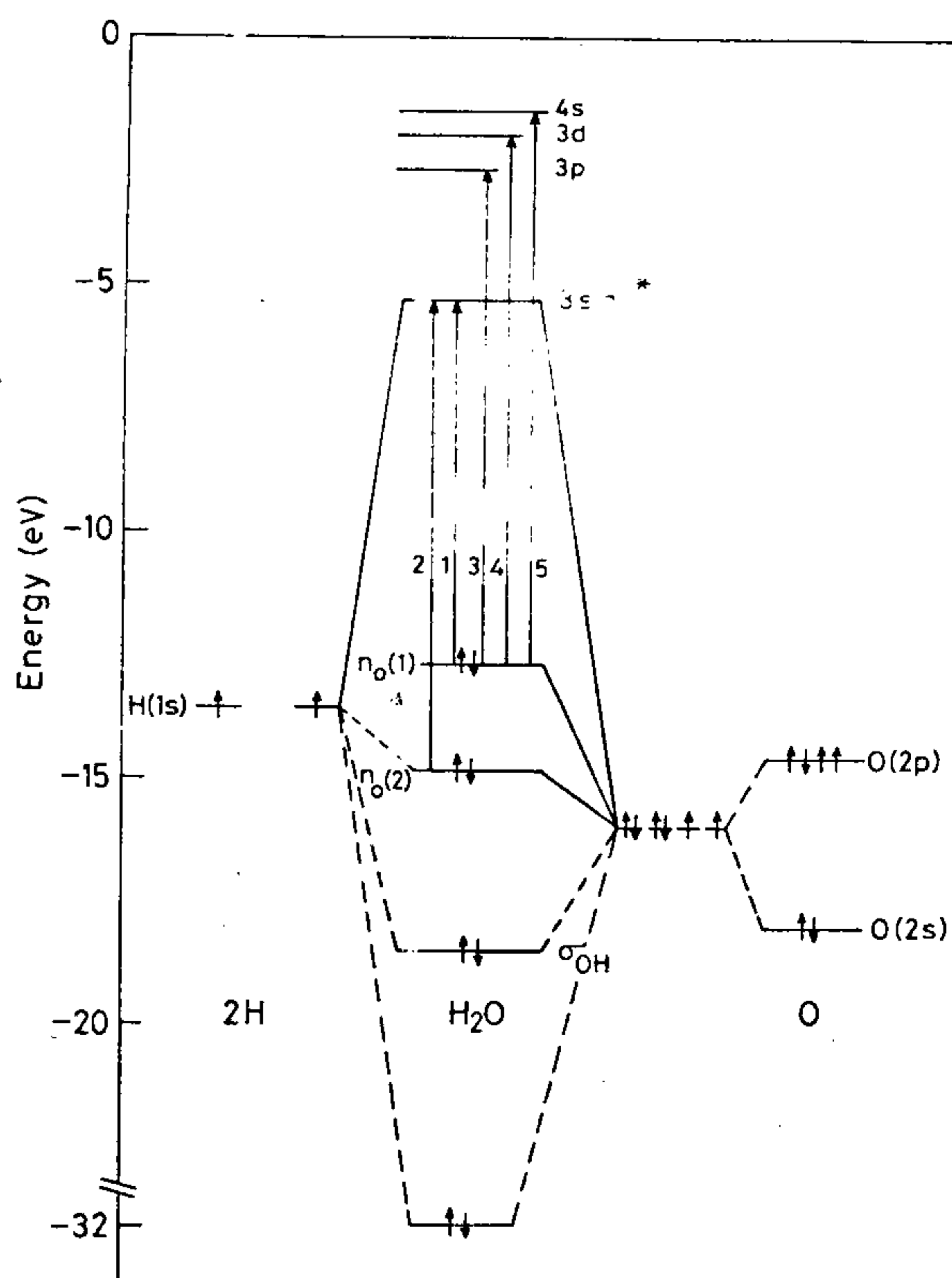
Figure 6. Electron states of H 2 O molecule.
