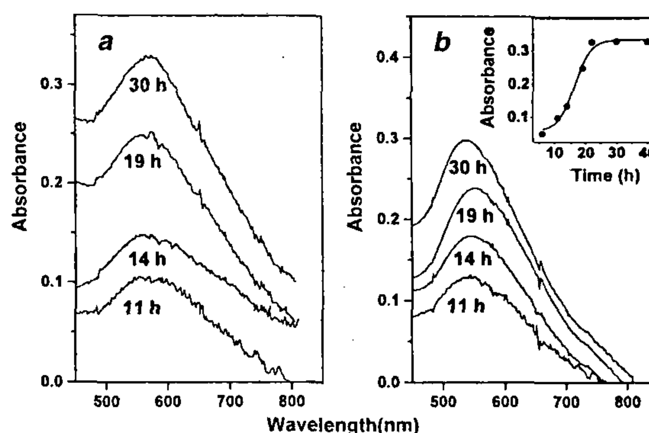
Figure 7. a, UV-vis spectra measured ex-situ of 130 Å colloidal gold-ODA composite films as a function of time of immersion of the ODA film in the colloidal solution (the time of immersion is indicated next to the corresponding curves); b, UV-vis spectra measured in-situ of 130 Å colloidal gold-ODA composite films as a function of time of immersion of the ODA film in the colloidal solution (the time of immersion is indicated next to the corresponding curves). The inset shows a plot of the variation of the surface plasmon resonance intensity with time of immersion of the films shown in the main part of Figure 7b.
