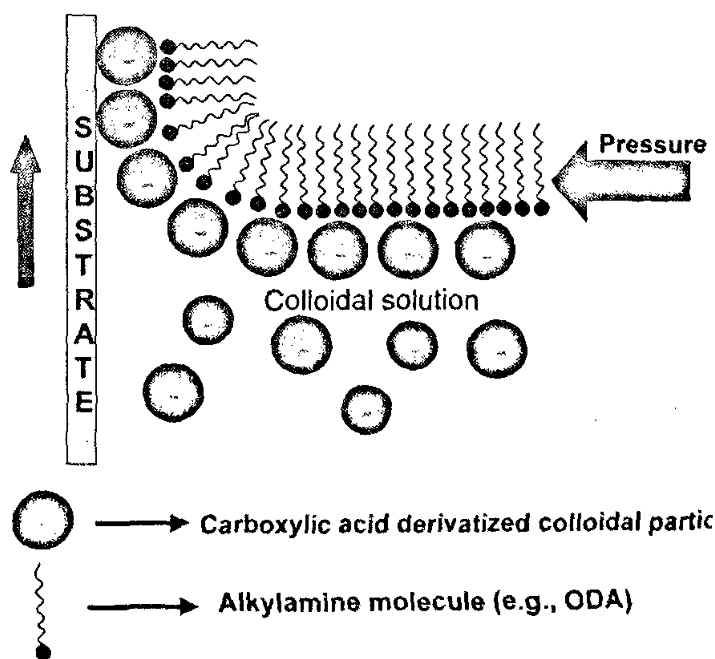
Scheme 4. Diagram showing the electrostatic immobilization of carboxylic acid derivatized colloidal nanoparticles at the air-water interface with positively charged ODA molecules and transfer thereafter of the nanoparticle monolayer onto suitable substrates by the LB technique.
