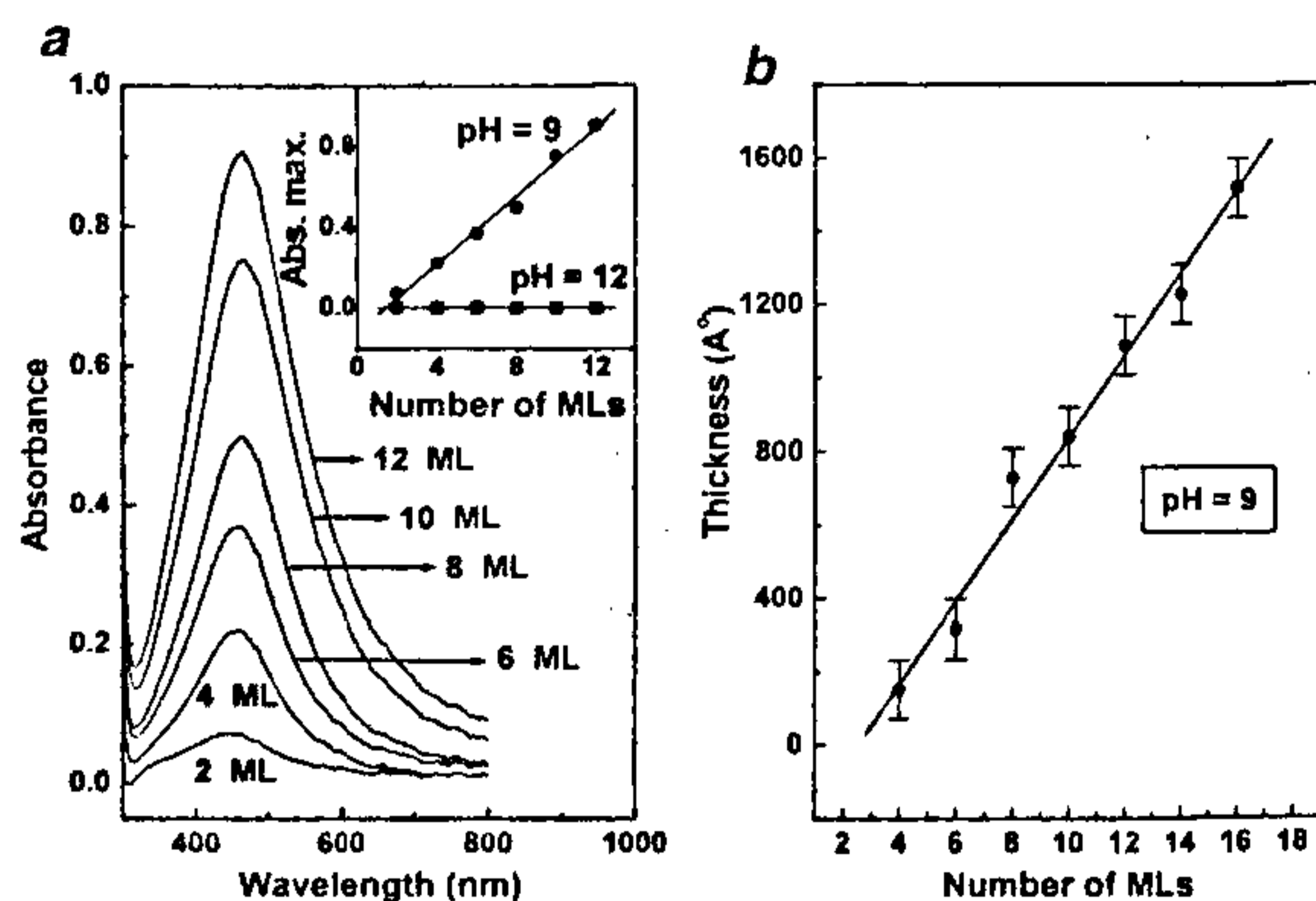
Figure 3. a , UV–vis spectra recorded from the silver colloidal particle LB films as a function of thickness of the films. The number of monolayers (ML) of the colloidal particles transferred onto quartz is indicated next to the respective curves. The inset shows a plot of the intensity of the plasmon resonance with thickness of silver particle LB film for the films grown from the pH = 9 and 12 subphases; b , Thickness of LB films of colloidal silver particles estimated from optical interferometry measurements as a function of number of monolayers transferred at pH = 9.
