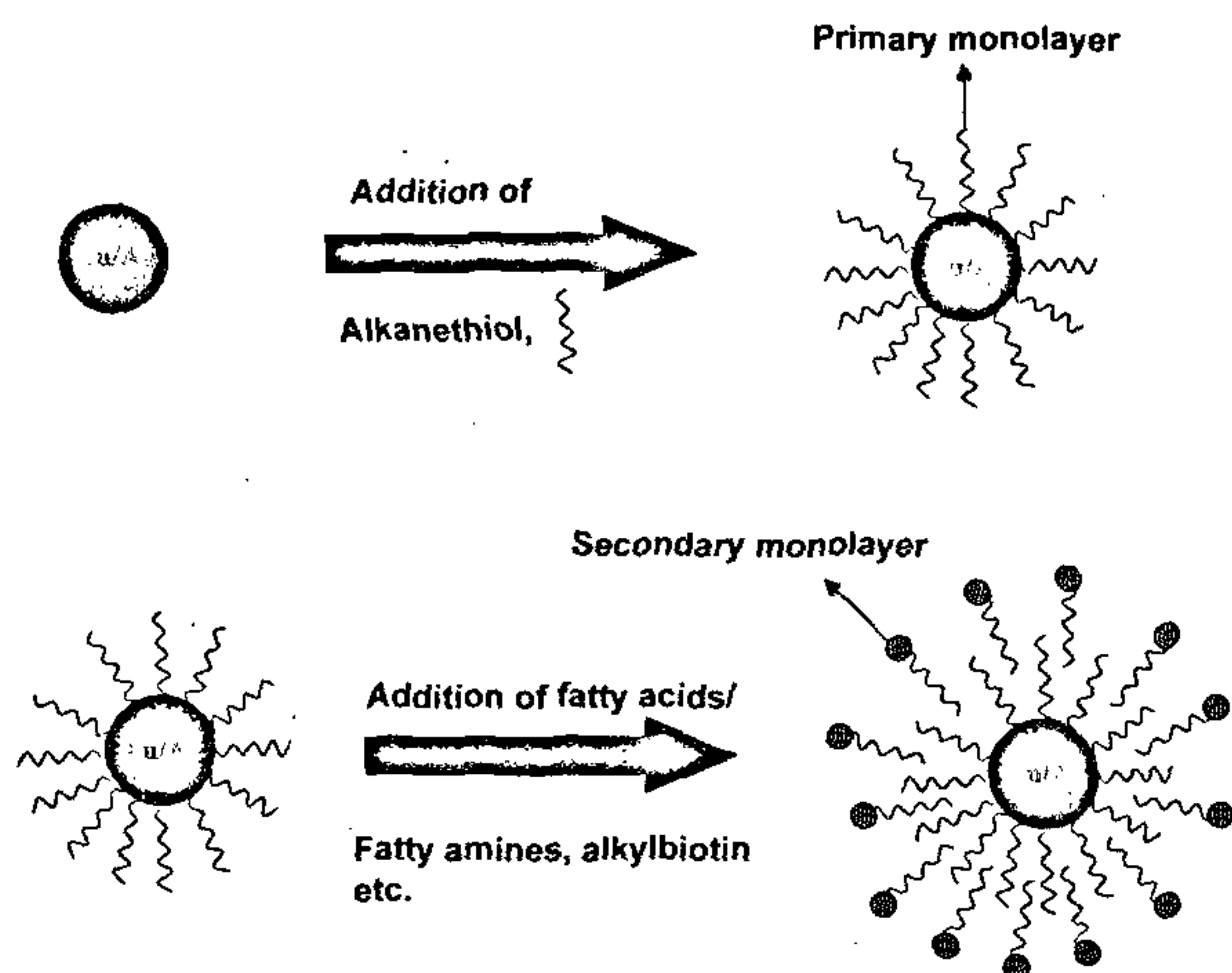
Scheme 3. Surface modification of colloidal nanoparticles via interdigitated bilayer formation. The various steps in the surface-modification procedure are illustrated.
