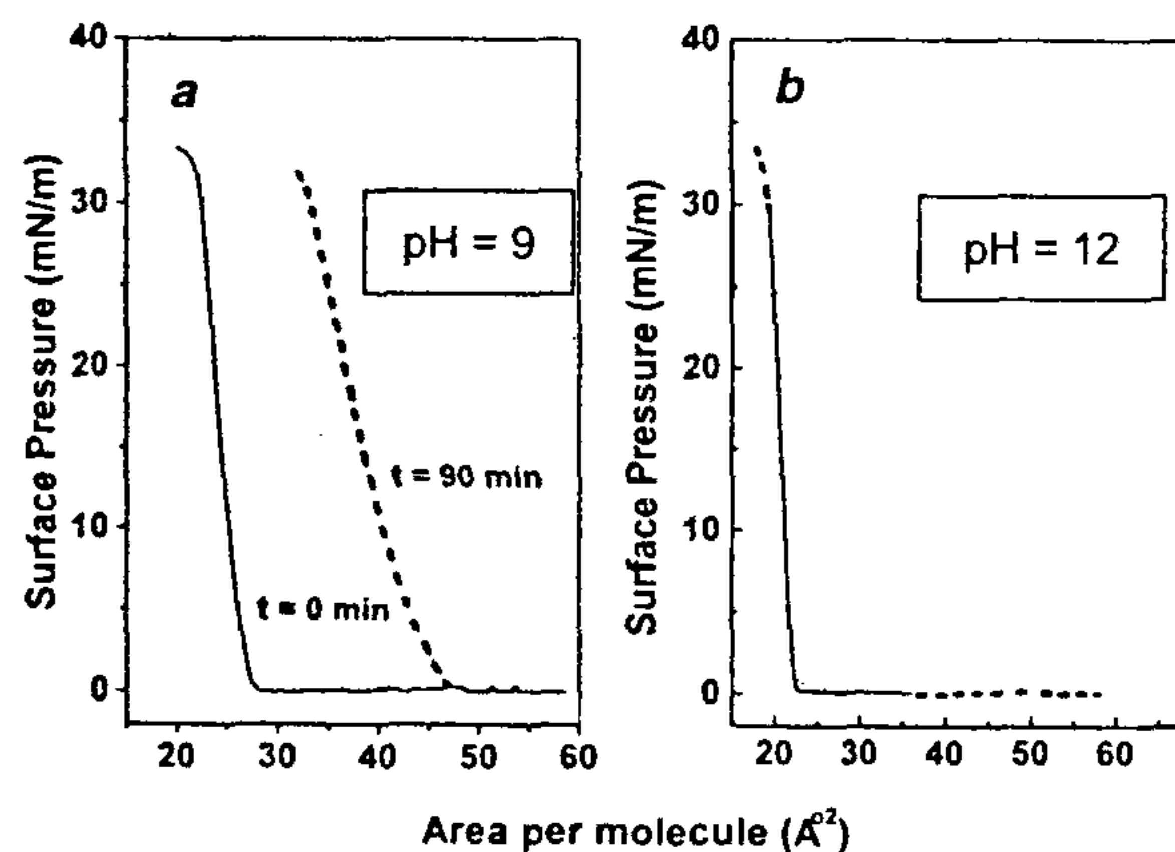
Figure 1. \pi - A isotherms of ODA monolayers spread on carboxylic acid derivatized colloidal silver solution at (a) \text{pH} = 9 and (b) \text{pH} = 12 , recorded as a function of time of spreading the monolayer (solid line, t = 0 min and dashed line, t = 90 min).
