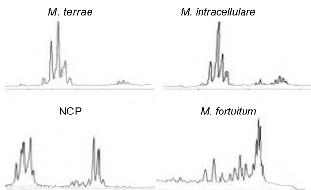
Figure 1. Representative chromatograms.
