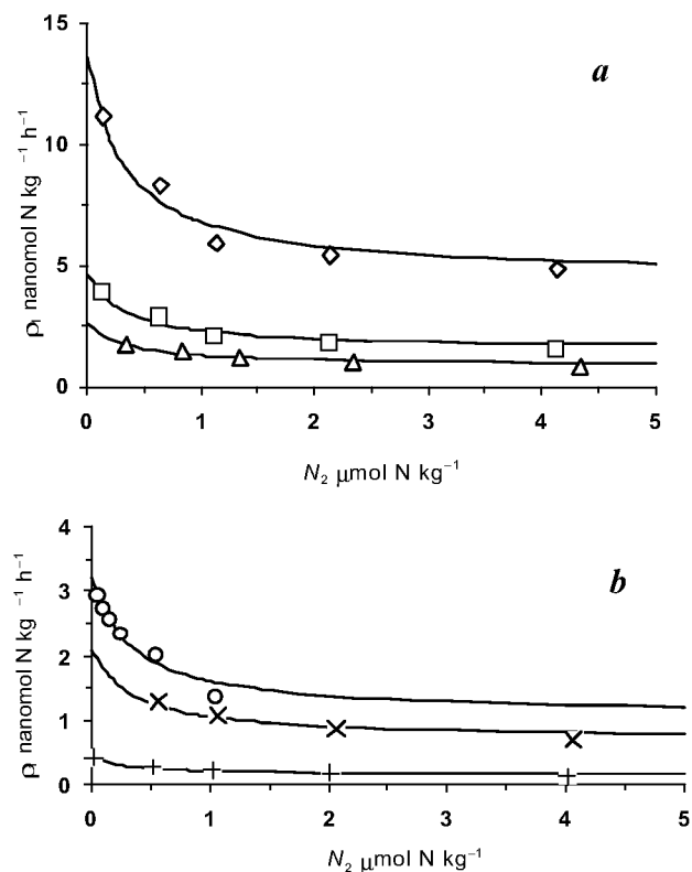
Figure 4 a and b. Nitrate uptake vs ammonium concentration: Comparison of values calculated using the eq. (8) (—) with experimental data. a_{12} = 1 , b_{12} = 3 . Values of nitrate uptake in the absence of ammonium are given in Table 1. Notation is as in Figure 1.
