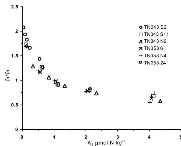
Figure 1. Normalized nitrate uptake vs ammonium concentration in the experiments of McCarthy et al. 1 . N_1^i = 1 \mu\text{M} . The experiments were performed on the cruises TN043 and TN053 during the NE monsoon in 1995. Notation for JGOFS stations is as in McCarthy et al. 1 .
