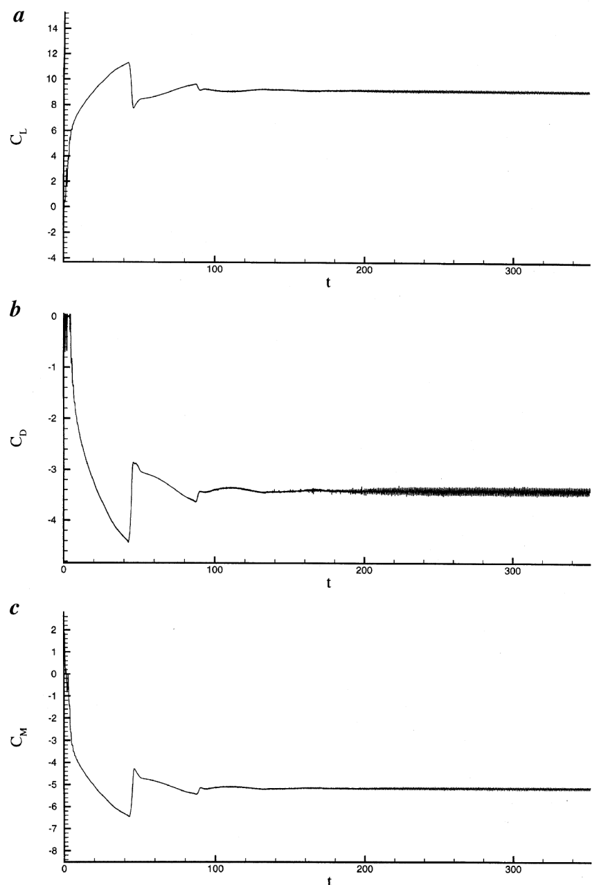
Figure 2. Loads and moment co-efficients variation with time for Re = 3800 and \Omega = 5.0 : (a) lift co-efficient, (b) drag co-efficient and (c) pitching moment co-efficient.
