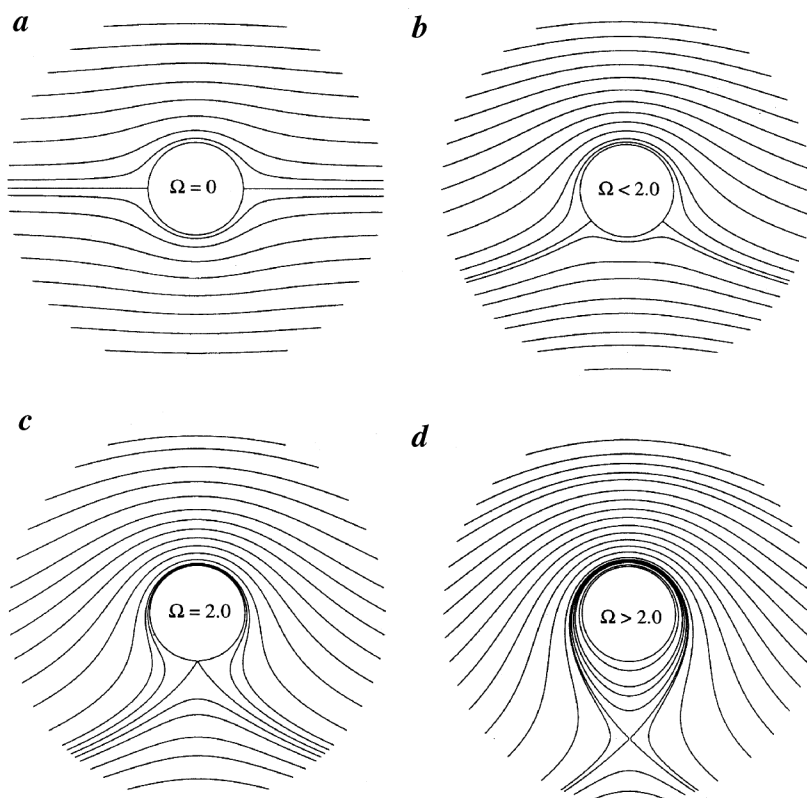
Figure 1. Inviscid irrotational flow past a rotating cylinder for (a) zero, (b) subcritical, (c) critical and (d) supercritical rotation rates.
