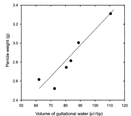
Figure 2. Relationship for six rice cultivars between the rate of guttation and their panicle weights (the yield sink potential). Y = 1.4718 + 0.1064x ( r = 0.94^{**} ).
