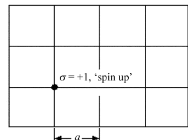
Figure 1. The square lattice \Gamma_a , lattice spacing a .
