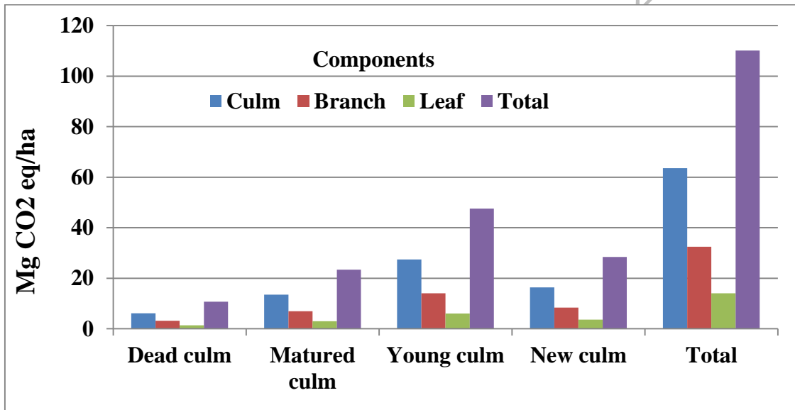
Figure-4: Carbon dioxide release abatement (Mg CO 2 eq ha -1 ) in bamboo plantation
