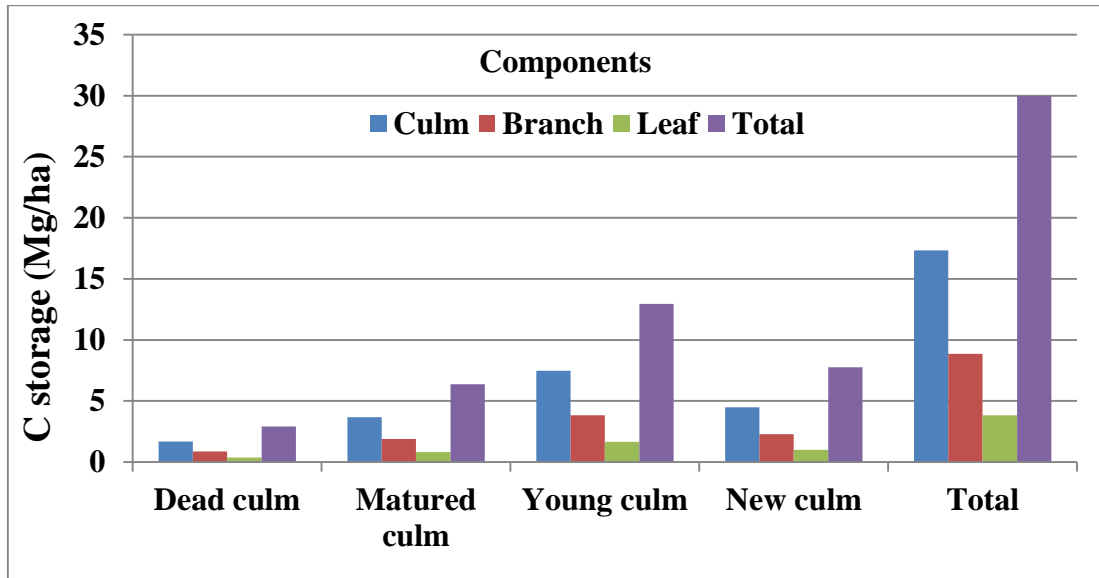
Figure-3: Carbon storage (Mg ha -1 ) in bamboo plantation
