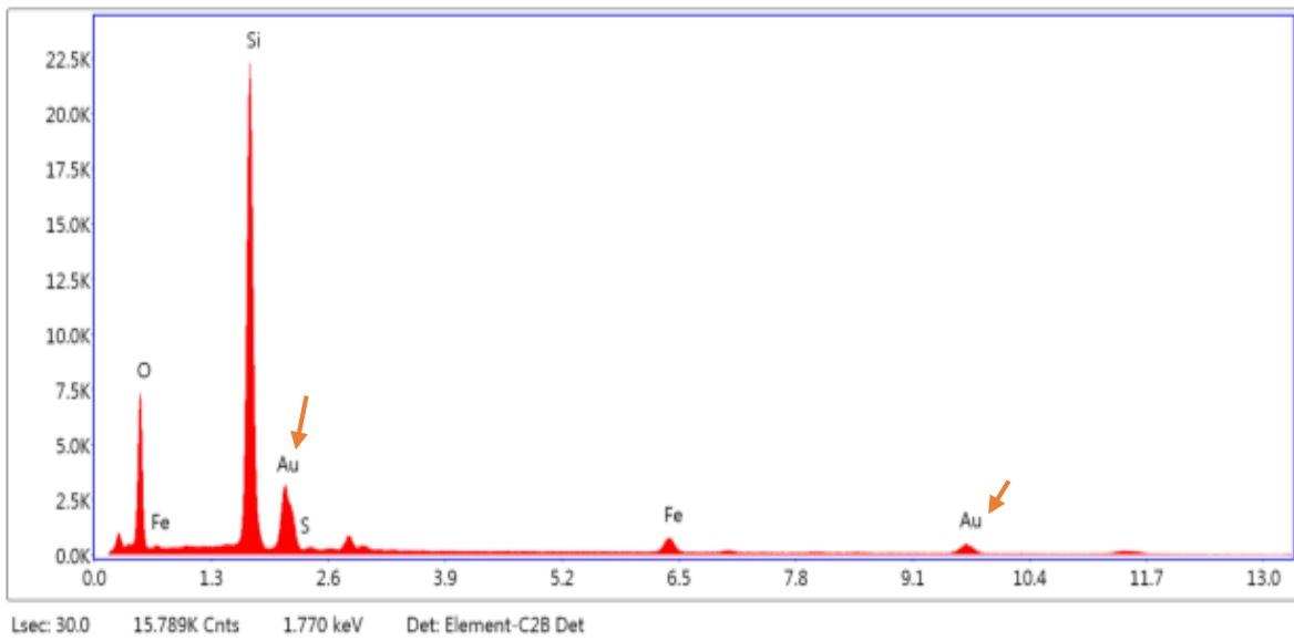
Figure 3. SEM-EDS spectrum of heavy fraction with presumptive gold sulfide grains. The peaks indicating presence of the elemental gold and Sulphur can be seen in the spectrum
