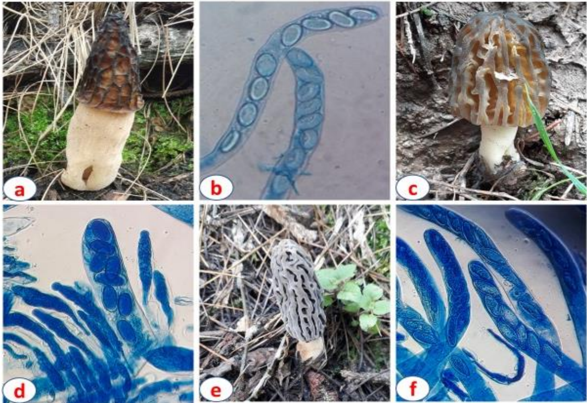
Plate. 2. Fig. a-f: Morchella elata Fr. Fig. a. Honey comb shaped black to brown fruiting body showing pileus and long stipe; Fig. b. Asci with ascospores (400x); Morchella kaibabensis Beug, T. A. Clem. & T. J. Baroni: Fig. c. Fruiting body showing pileus having long pits and creamish stipe; Fig. d. Asci with eight ascospores (400x); Morchella tridentina Bres.: Fig. e. Conical ascocarp showing pileus and short stipe; Fig. f. Asci with eight ellipsoidal ascospores (400x).
