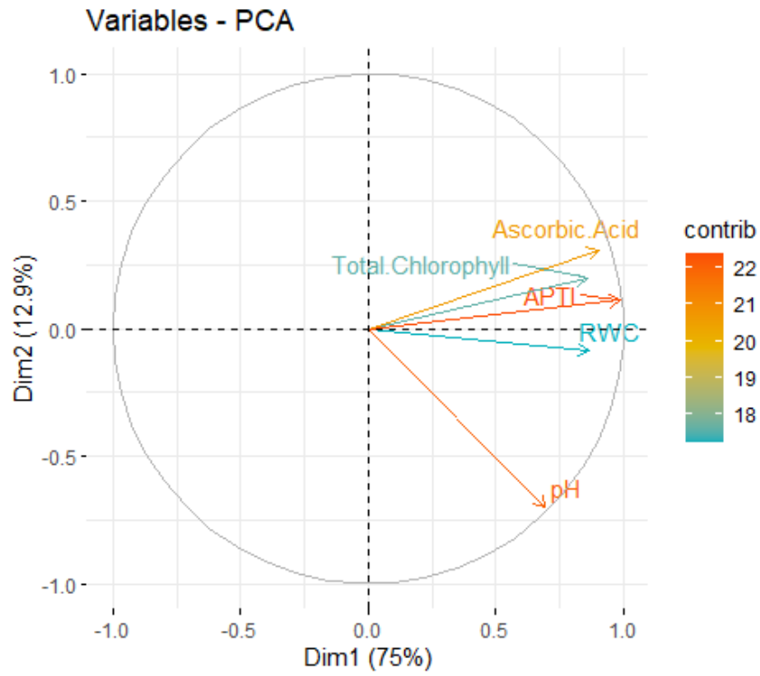
Figure 3: Principal component analysis signifying contribution of different air pollutants
