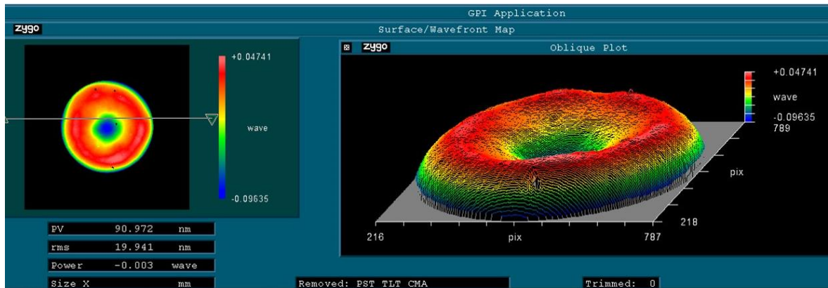
Fig. 6. Surface figure measurement data on M3 mirror using a Zygo make optical interferometer.
